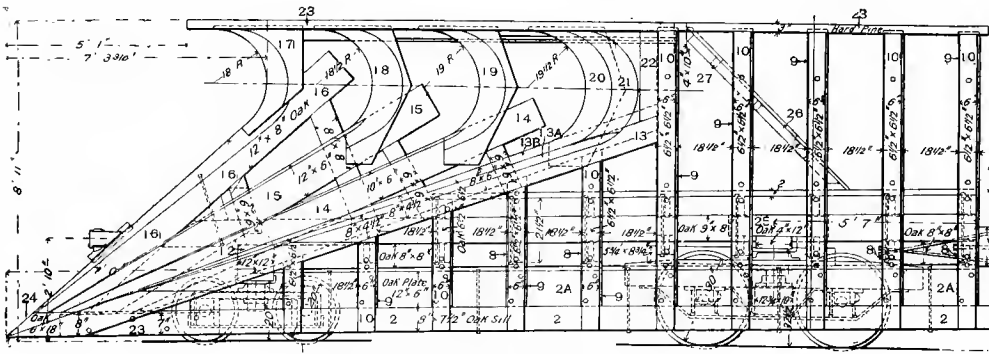
Fig. 410. Side Elevation of Framing.
